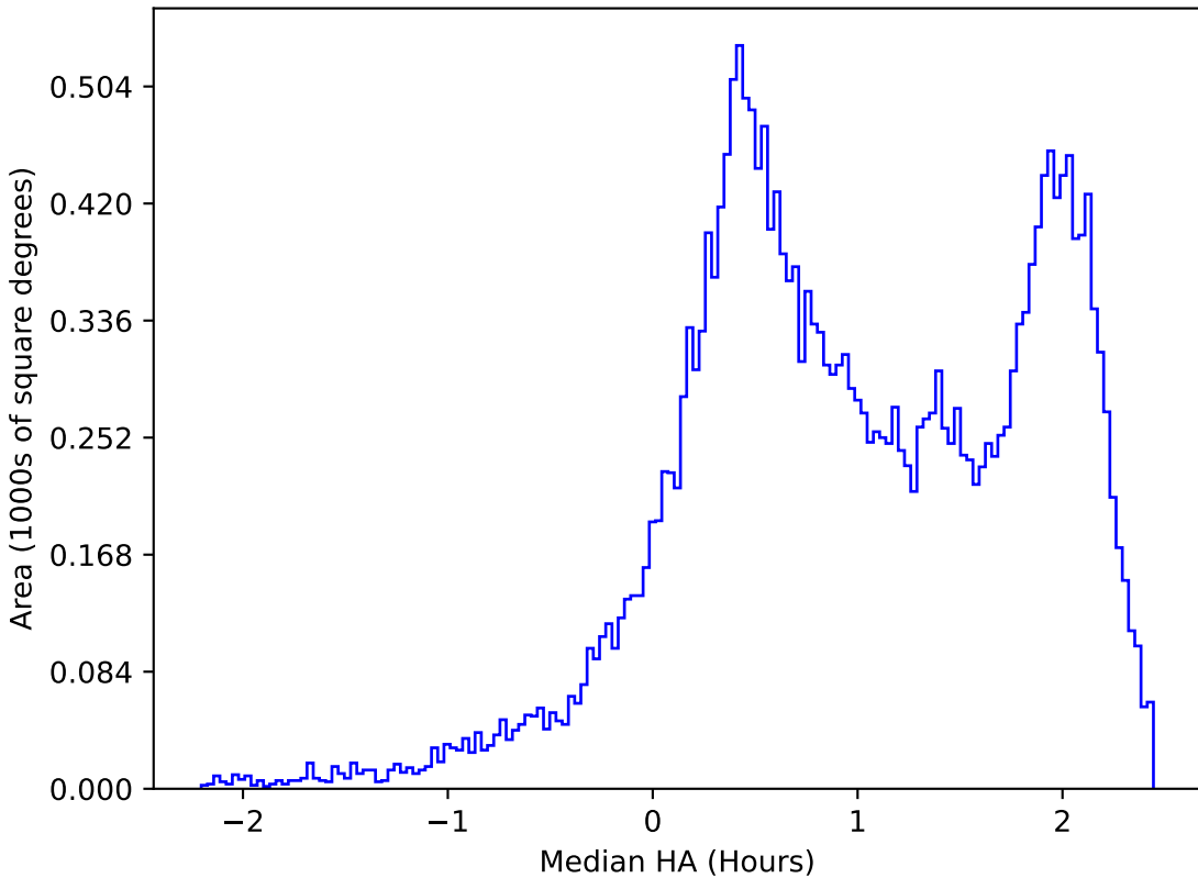
too_5_4v3.4_10yrs All sky z band: Median HA
