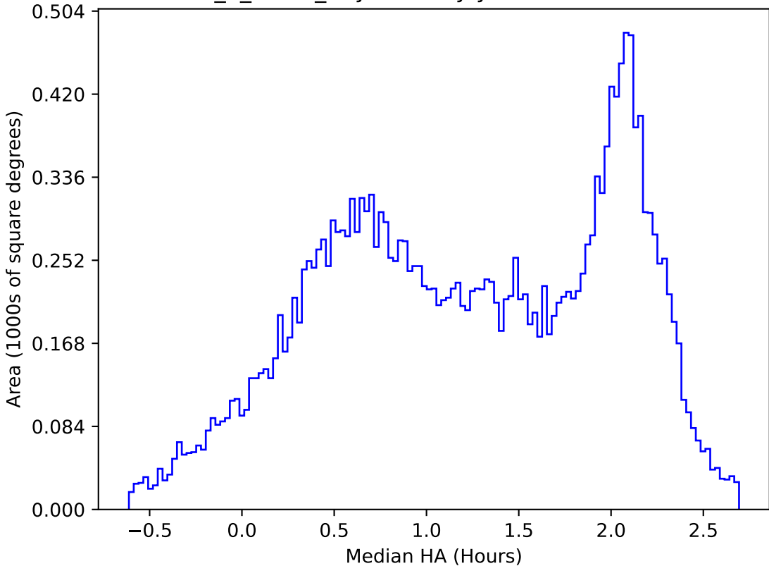
too_5_4v3.4_10yrs All sky y band: Median HA
