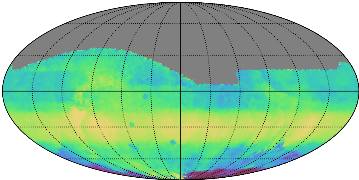
too_5_4v3.4_10yrs All sky i band: Median HA
