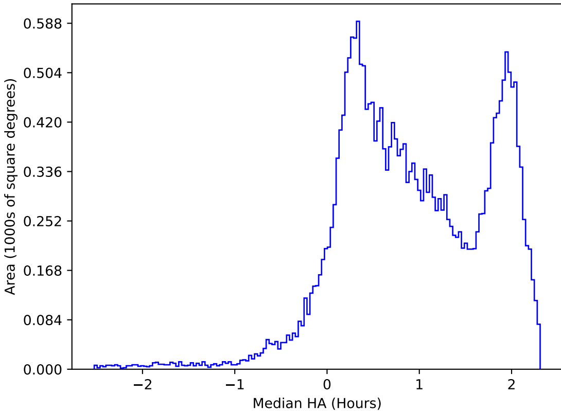
too_5_4v3.4_10yrs All sky i band: Median HA
