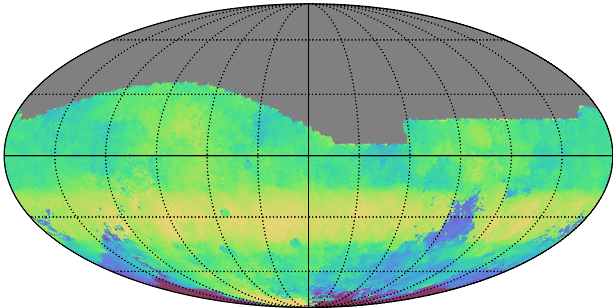
too_5_4v3.4_10yrs All sky g band: Median HA
