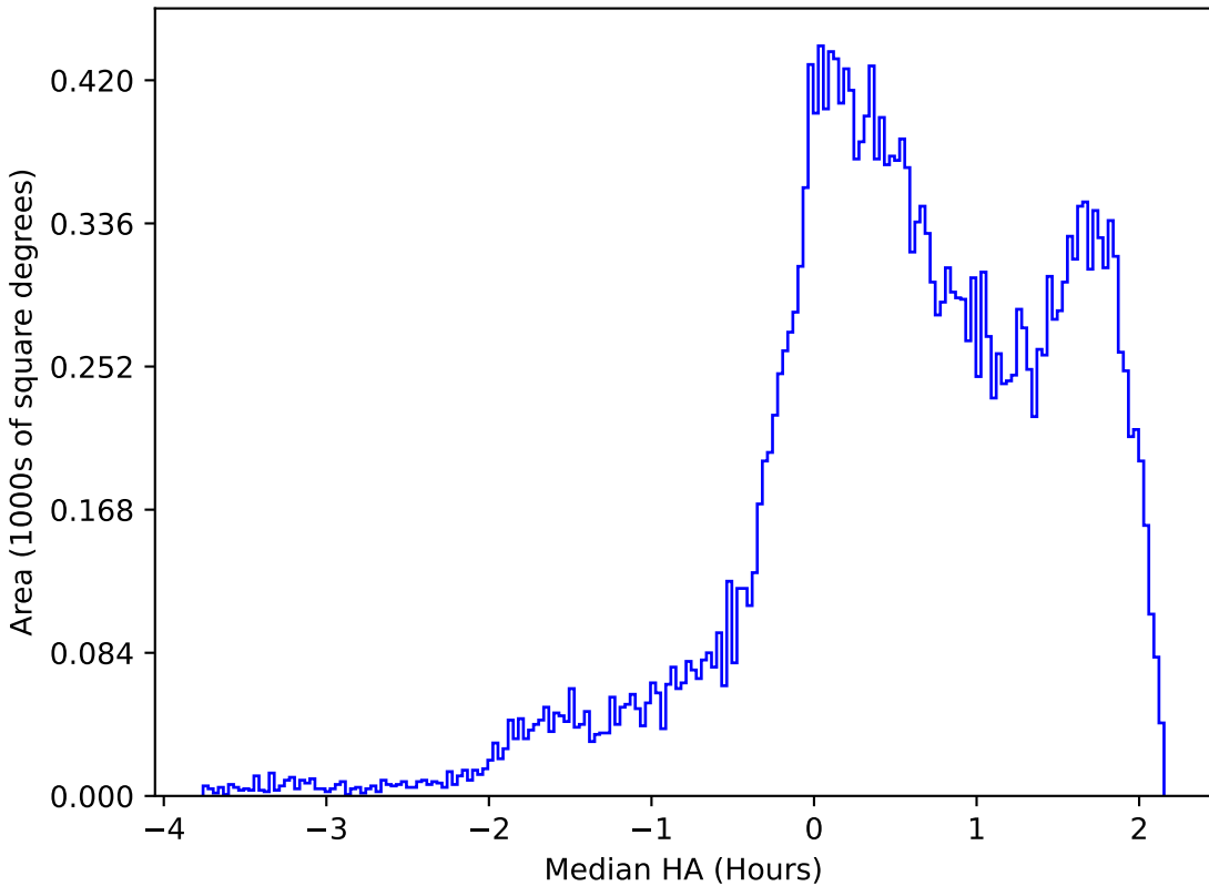
too_5_4v3.4_10yrs All sky g band: Median HA
