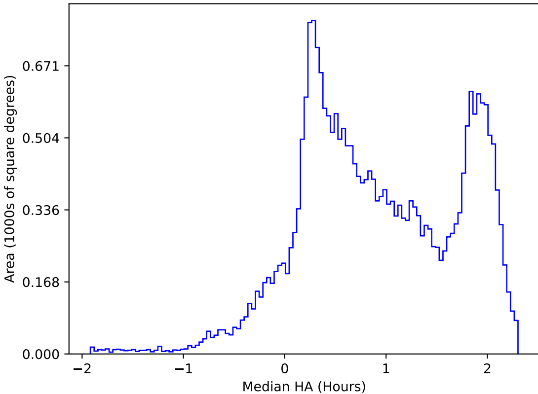
too_5_4v3.4_10yrs All sky all bands: Median HA
