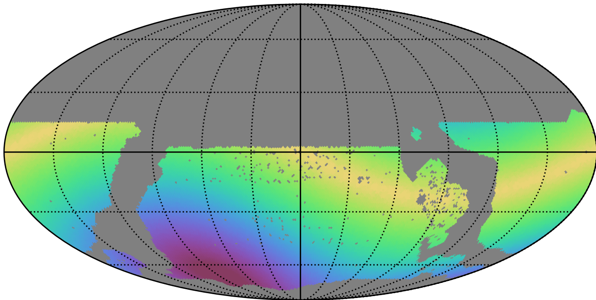
too_5_4v3.4_10yrs WFD z band: Max solarElong
