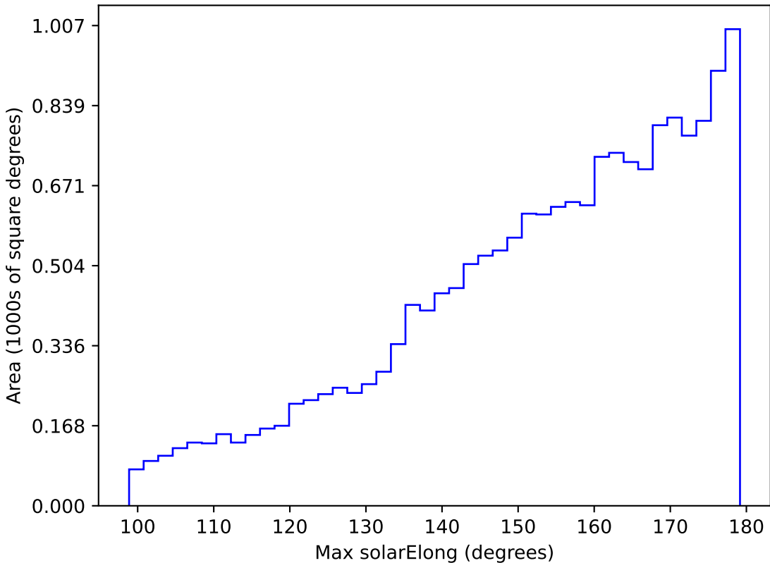
too_5_4v3.4_10yrs WFD y band: Max solarElong
