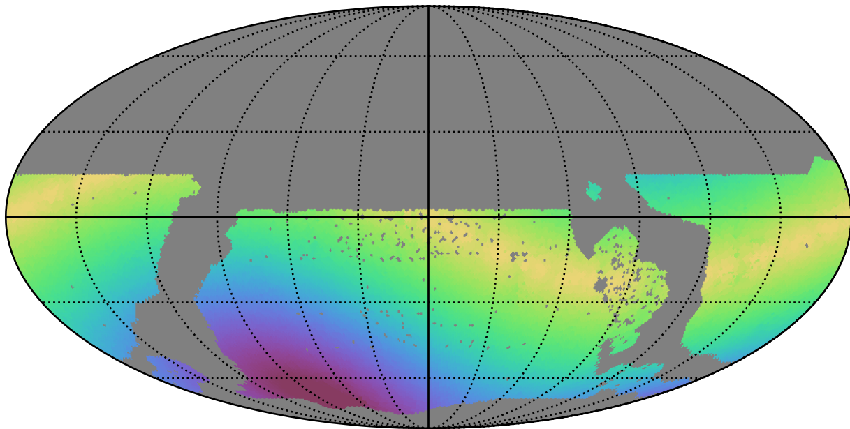
too_5_4v3.4_10yrs WFD u band: Max solarElong
