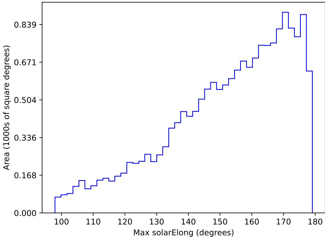
too_5_4v3.4_10yrs WFD u band: Max solarElong
