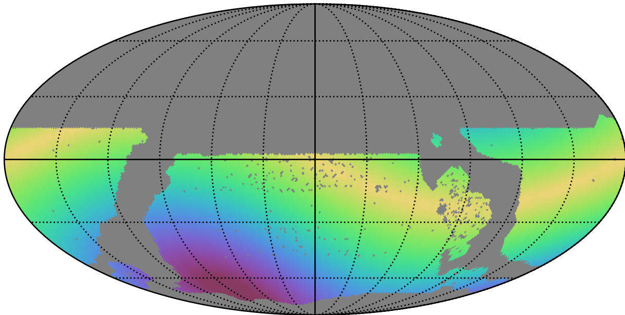
too_5_4v3.4_10yrs WFD r band: Max solarElong
