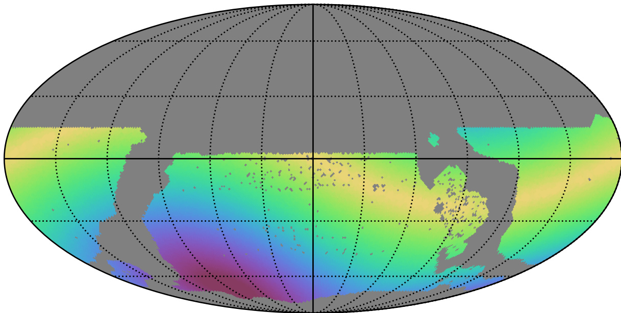
too_5_4v3.4_10yrs WFD i band: Max solarElong
