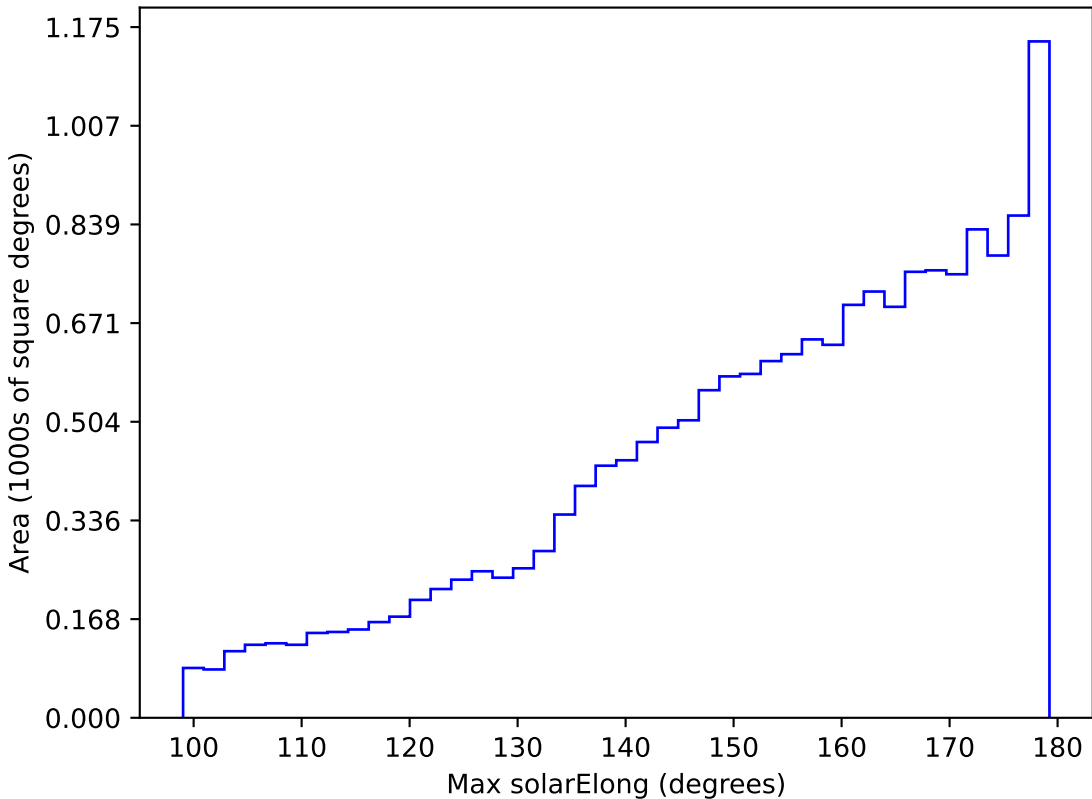
too_5_4v3.4_10yrs WFD i band: Max solarElong
