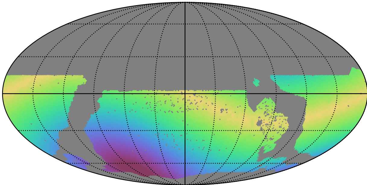
too_5_4v3.4_10yrs WFD g band: Max solarElong
