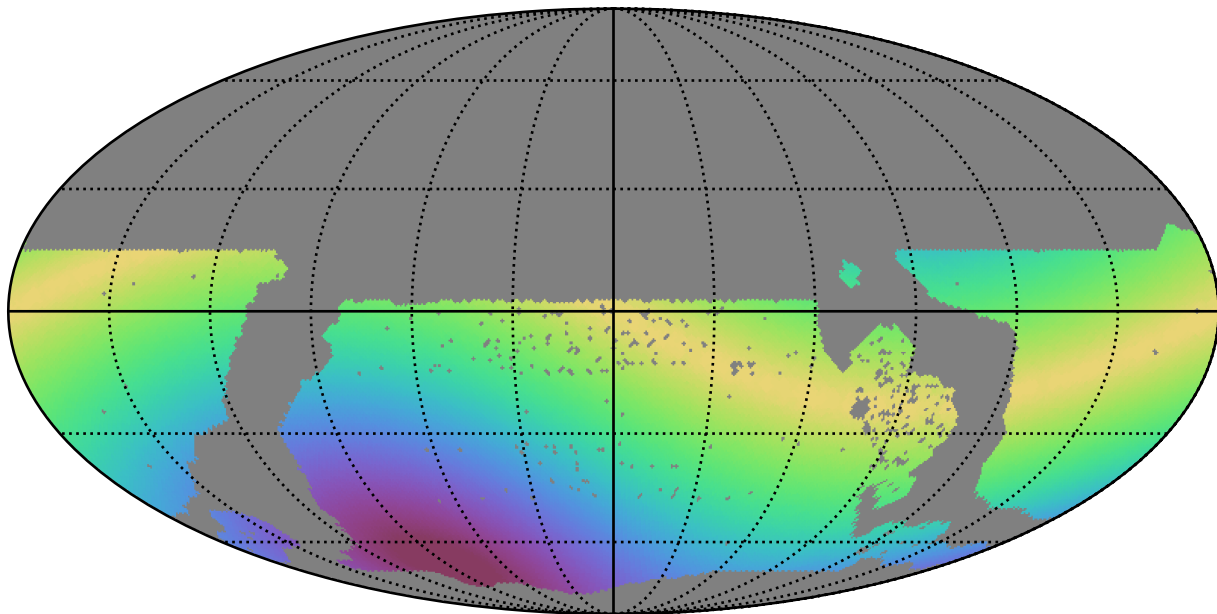
too_5_4v3.4_10yrs WFD all bands: Max solarElong
