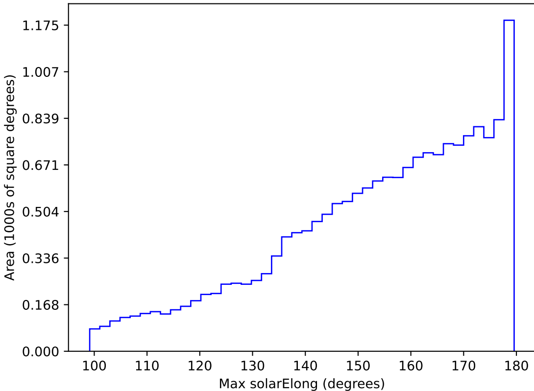
too_5_4v3.4_10yrs WFD all bands: Max solarElong
