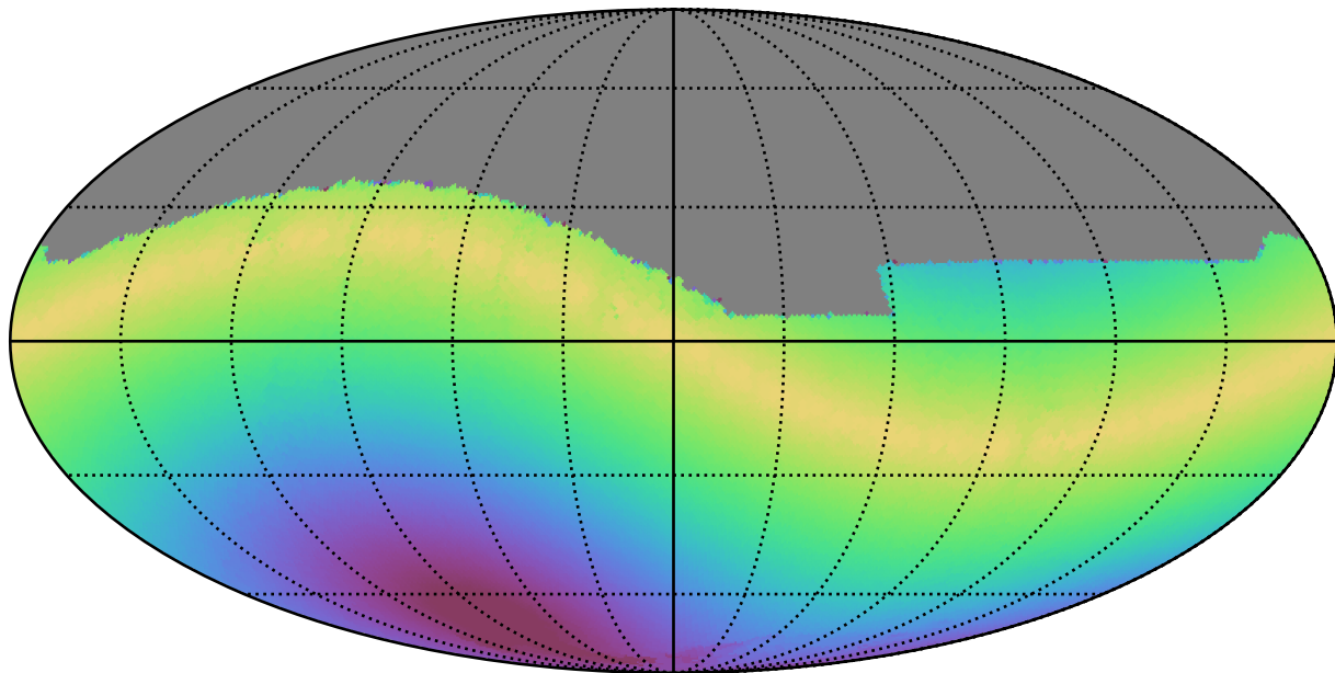
too_5_4v3.4_10yrs All sky z band: Max solarElong
