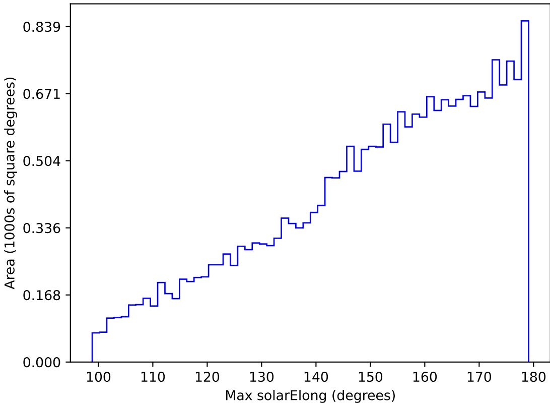
too_5_4v3.4_10yrs All sky y band: Max solarElong
