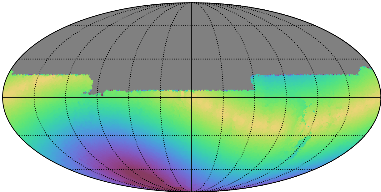
too_5_4v3.4_10yrs All sky u band: Max solarElong
