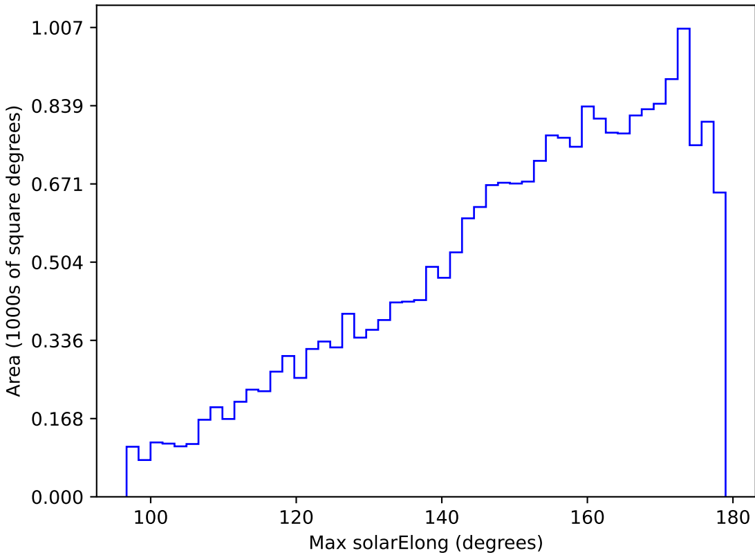
too_5_4v3.4_10yrs All sky u band: Max solarElong
