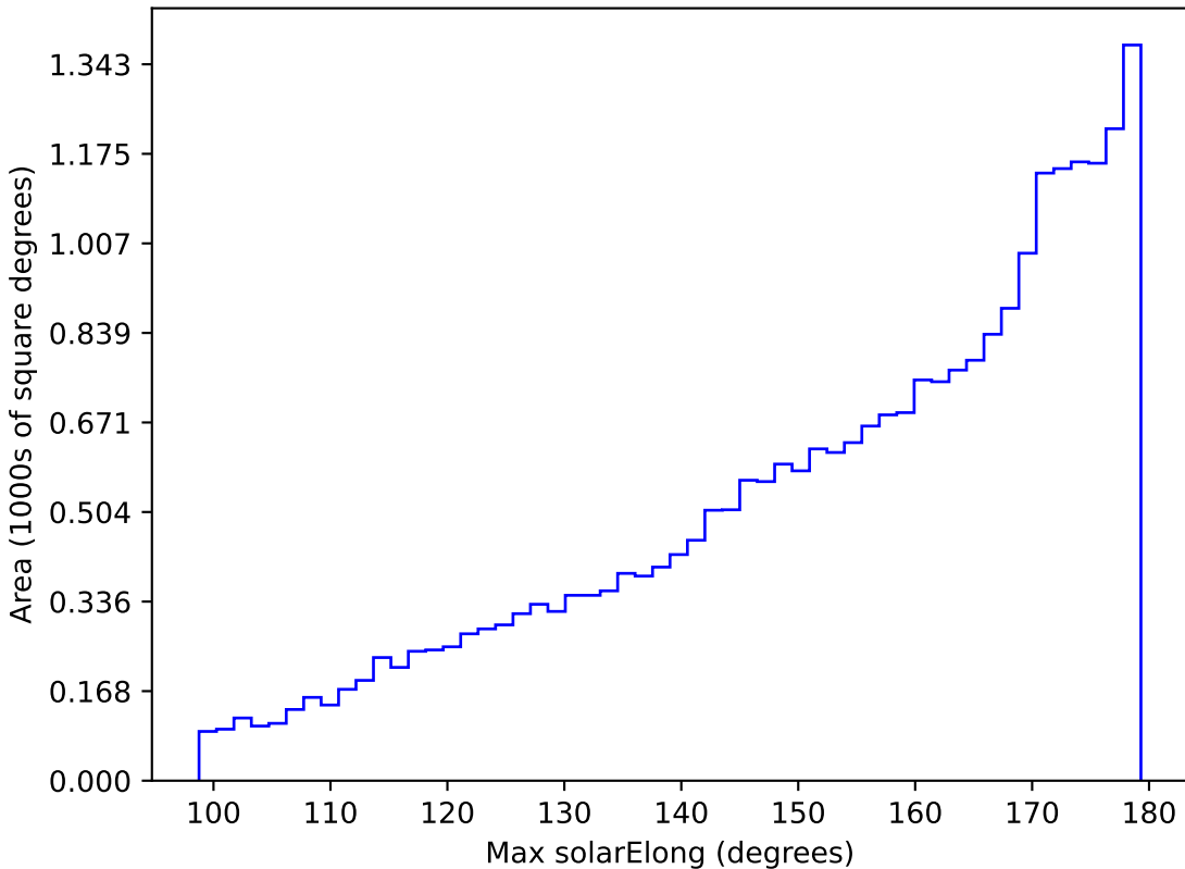
too_5_4v3.4_10yrs All sky r band: Max solarElong
