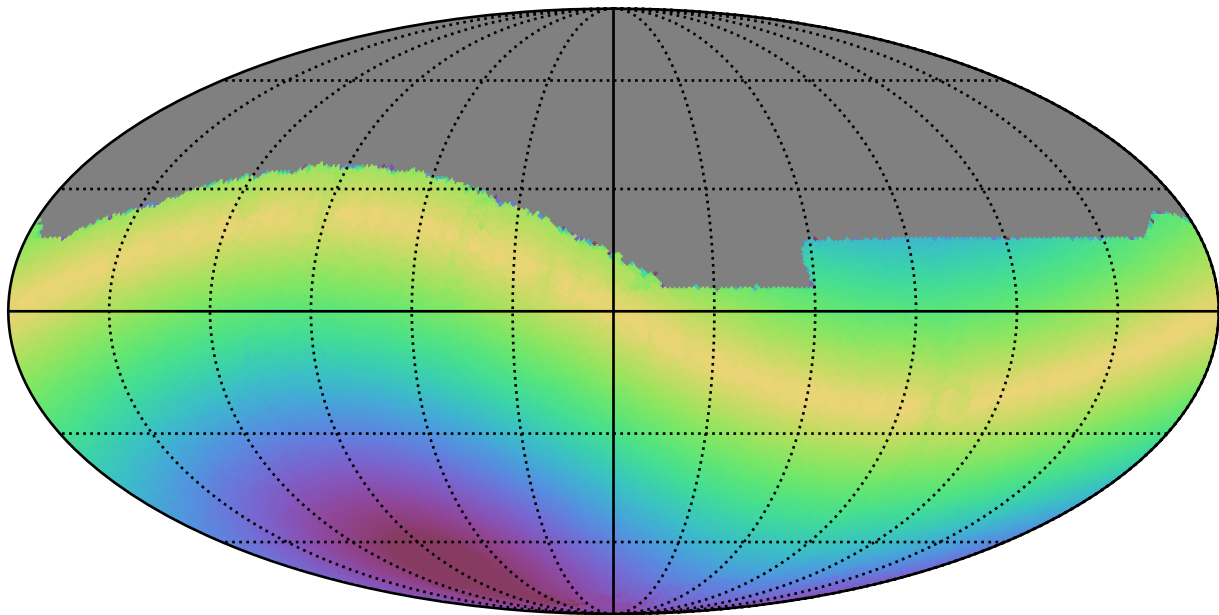
too_5_4v3.4_10yrs All sky i band: Max solarElong
