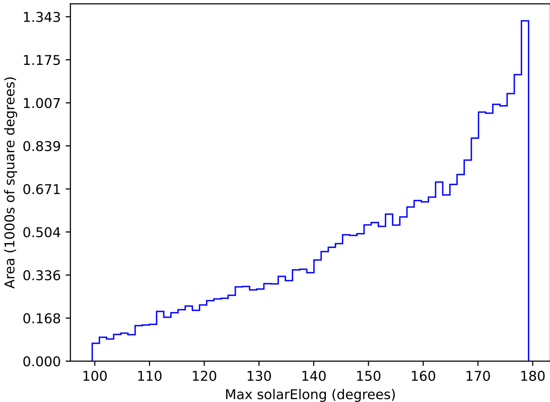
too_5_4v3.4_10yrs All sky i band: Max solarElong
