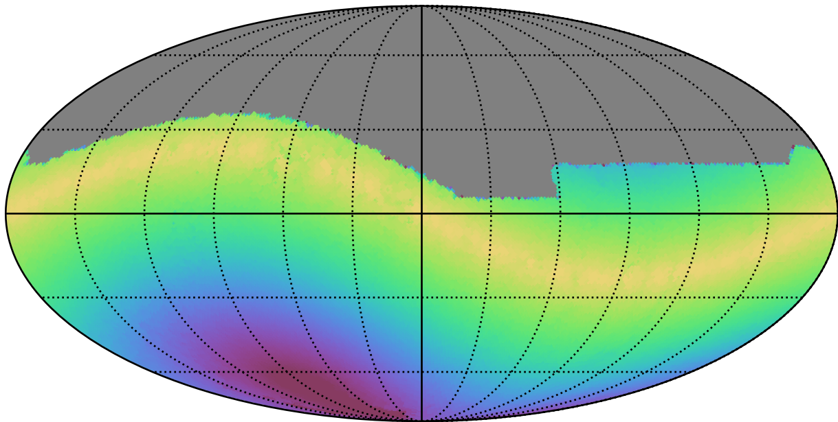
too_5_4v3.4_10yrs All sky g band: Max solarElong
