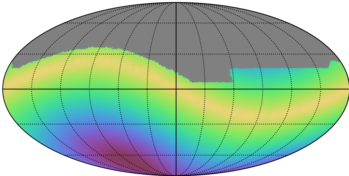
too_5_4v3.4_10yrs All sky all bands: Max solarElong
