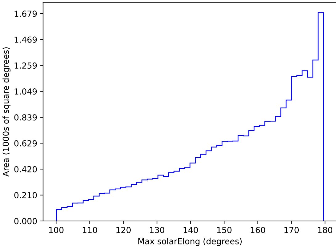
too_5_4v3.4_10yrs All sky all bands: Max solarElong
