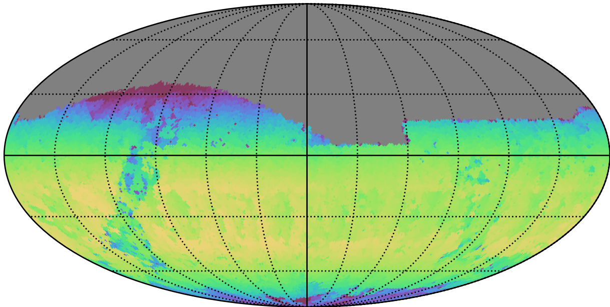
too_5_4v3.4_10yrs Yr 1 z band: Max skyBrightness
