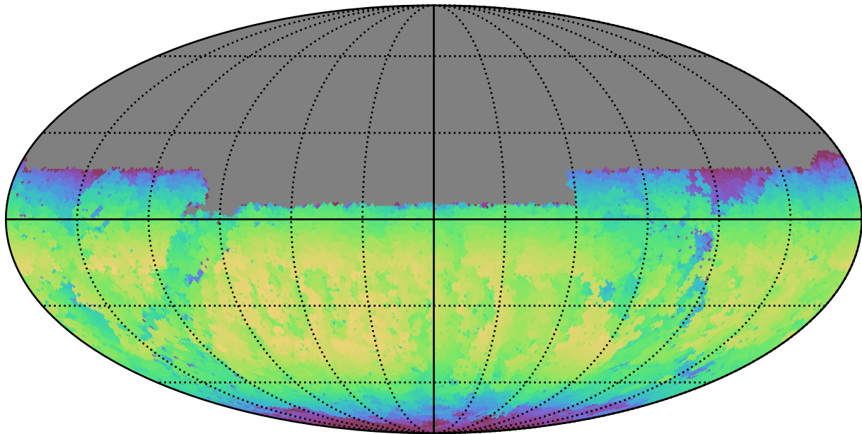
too_5_4v3.4_10yrs Yr 1 y band: Max skyBrightness
