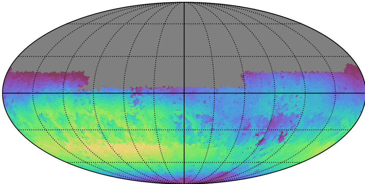
too_5_4v3.4_10yrs Yr 1 u band: Max skyBrightness
