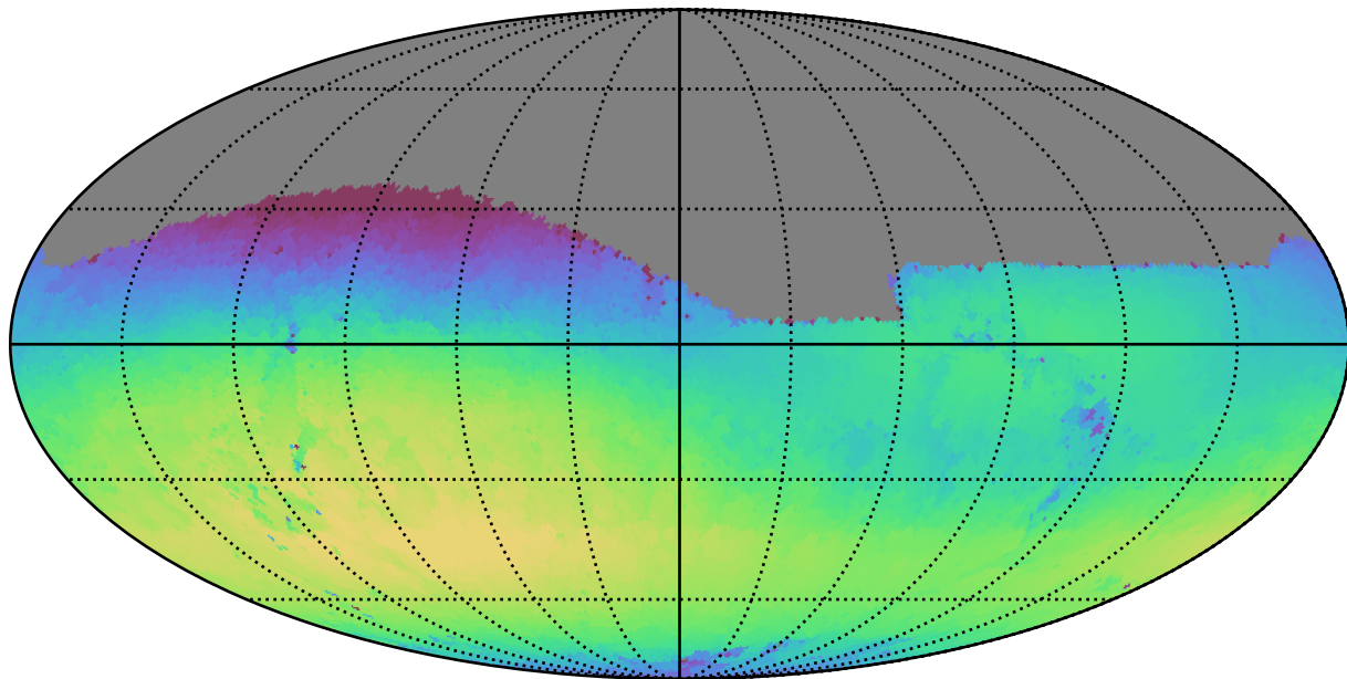
too_5_4v3.4_10yrs Yr 1 r band: Max skyBrightness
