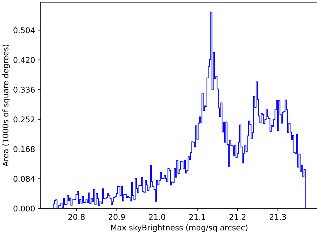
too_5_4v3.4_10yrs Yr 1 r band: Max skyBrightness
