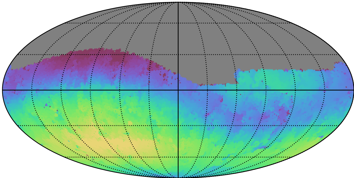
too_5_4v3.4_10yrs Yr 1 g band: Max skyBrightness
