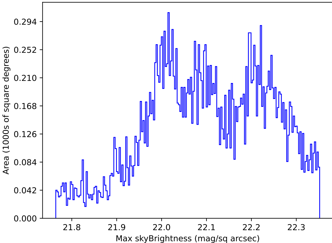
too_5_4v3.4_10yrs Yr 1 g band: Max skyBrightness
