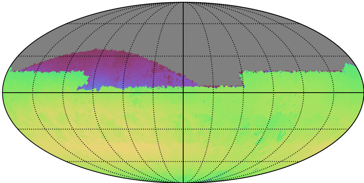
too_5_4v3.4_10yrs Yr 1 all bands: Max skyBrightness
