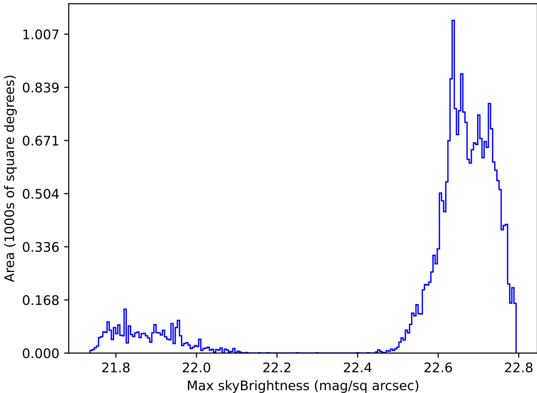
too_5_4v3.4_10yrs Yr 1 all bands: Max skyBrightness
