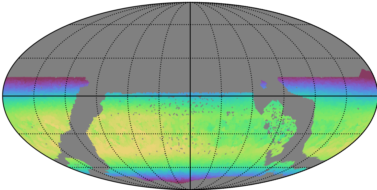
too_5_4v3.4_10yrs WFD z band: Max skyBrightness
