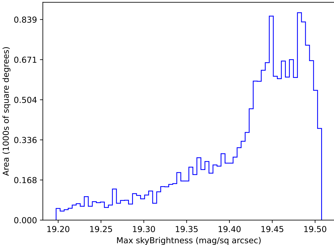
too_5_4v3.4_10yrs WFD z band: Max skyBrightness
