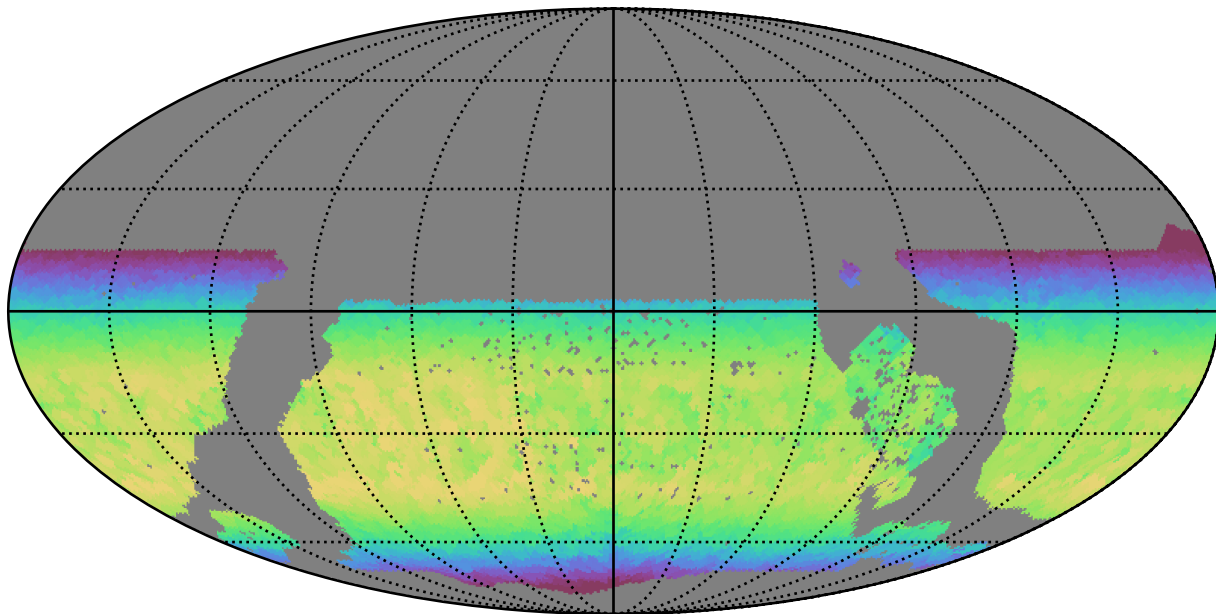
too_5_4v3.4_10yrs WFD y band: Max skyBrightness
