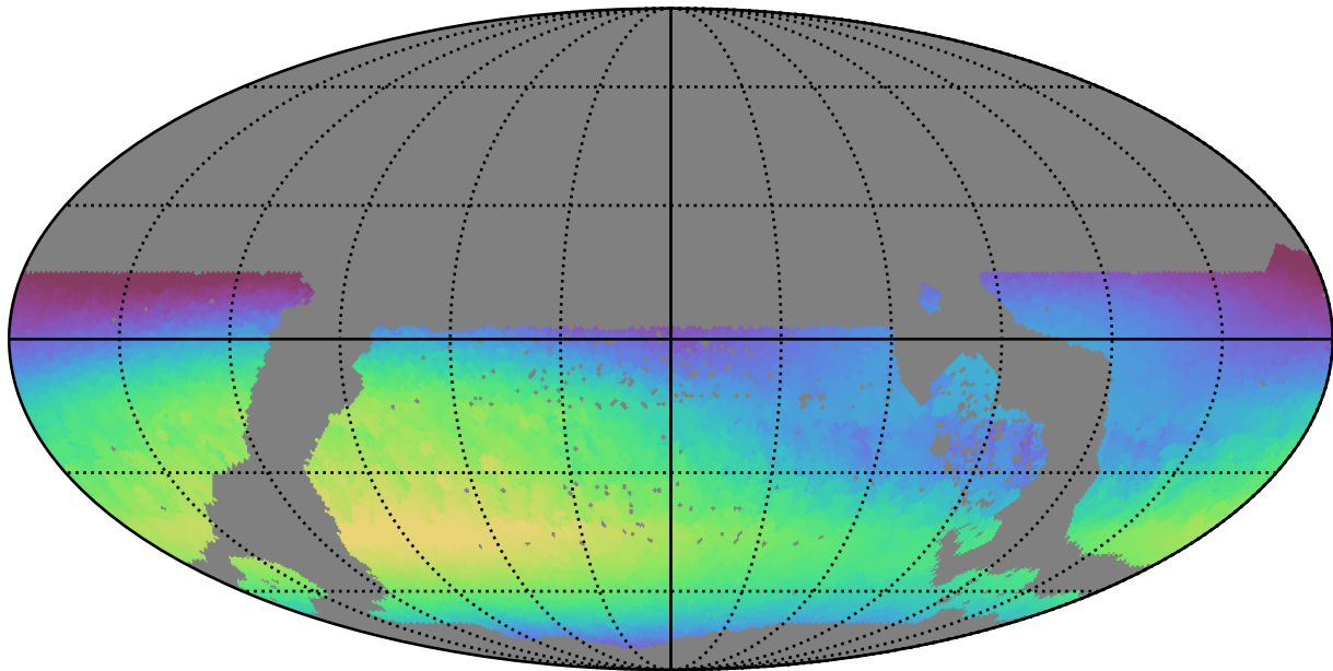
too_5_4v3.4_10yrs WFD u band: Max skyBrightness
