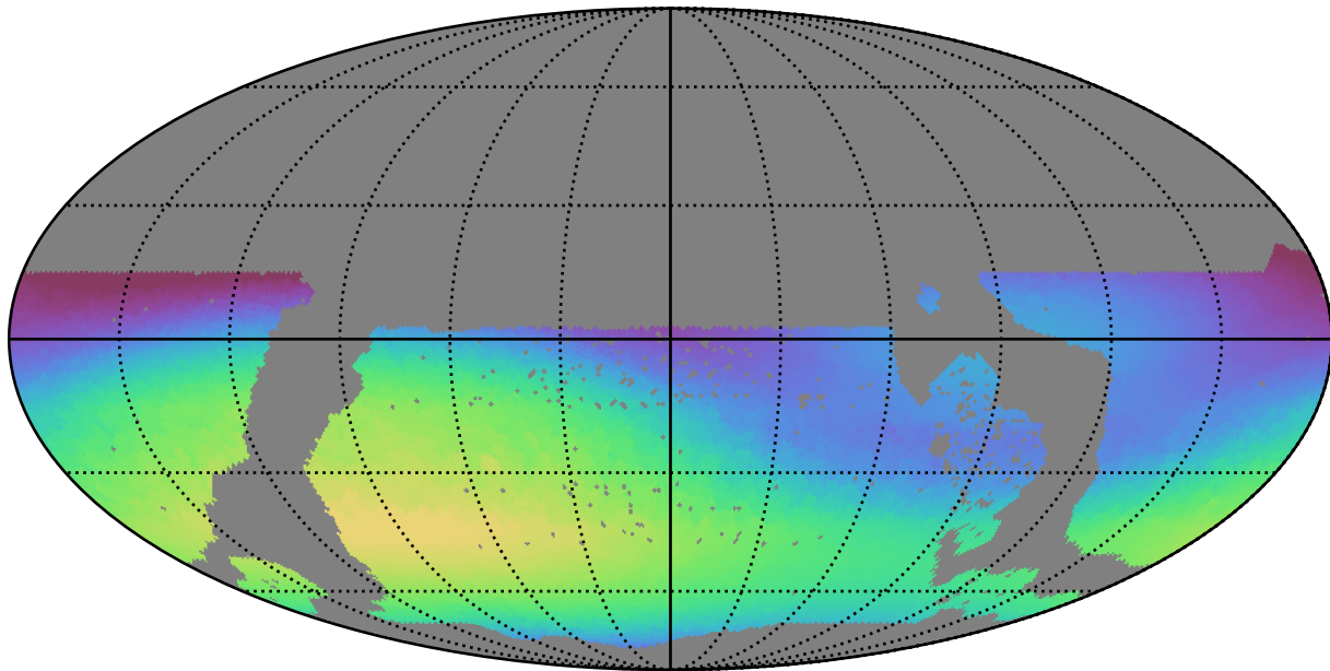
too_5_4v3.4_10yrs WFD r band: Max skyBrightness
