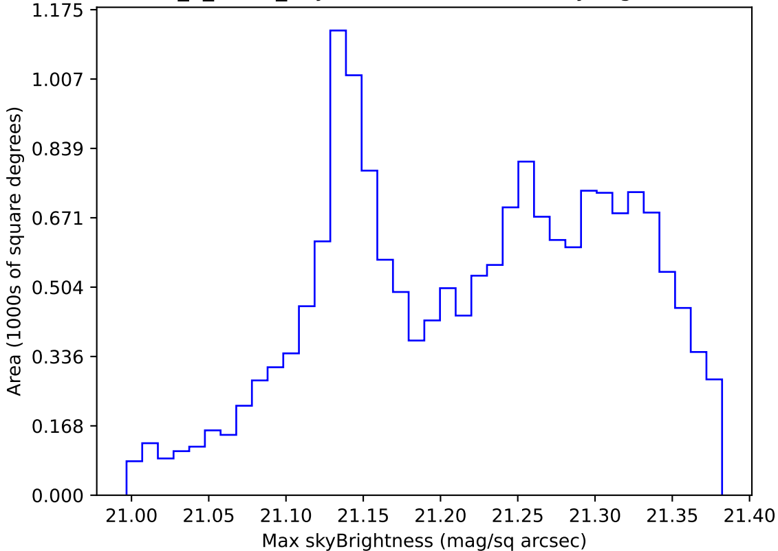
too_5_4v3.4_10yrs WFD r band: Max skyBrightness
