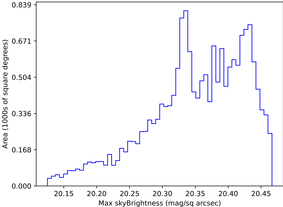
too_5_4v3.4_10yrs WFD i band: Max skyBrightness
