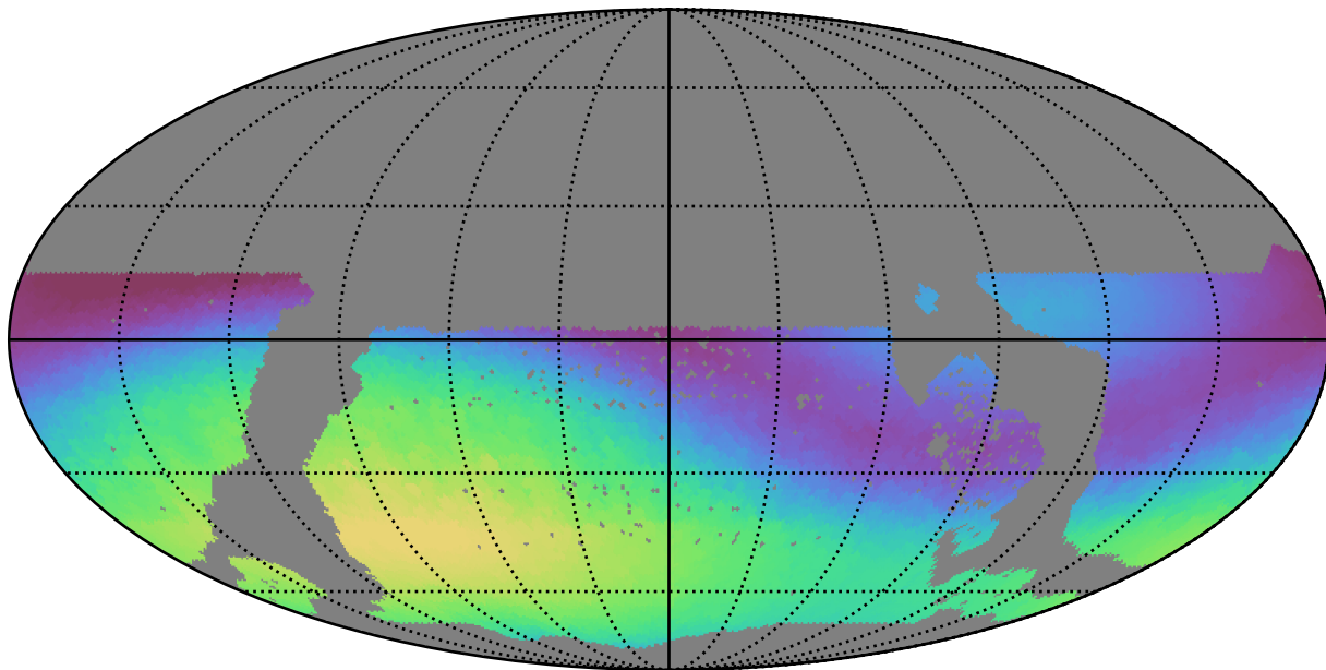
too_5_4v3.4_10yrs WFD g band: Max skyBrightness
