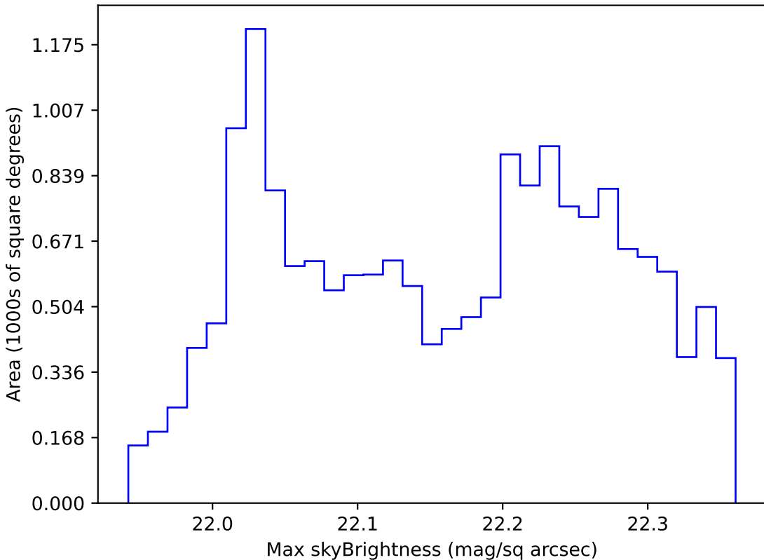
too_5_4v3.4_10yrs WFD g band: Max skyBrightness
