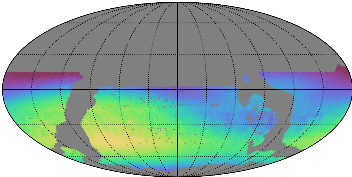
too_5_4v3.4_10yrs WFD all bands: Max skyBrightness
