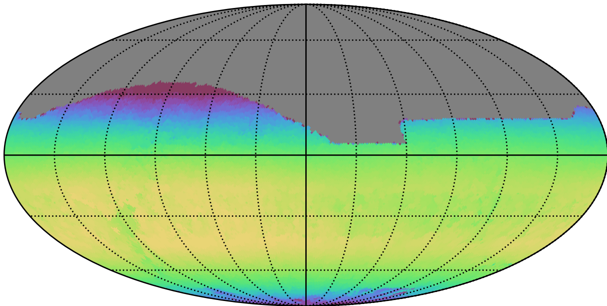
too_5_4v3.4_10yrs All sky z band: Max skyBrightness
