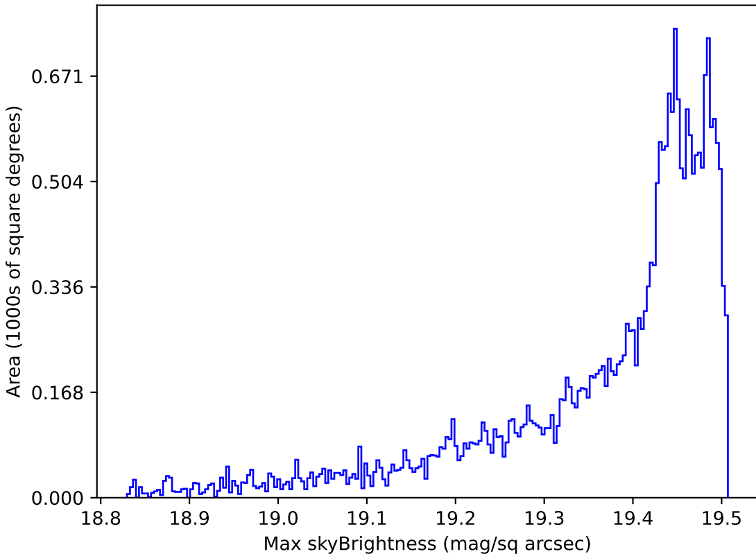
too_5_4v3.4_10yrs All sky z band: Max skyBrightness
