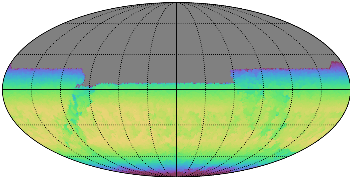
too_5_4v3.4_10yrs All sky y band: Max skyBrightness
