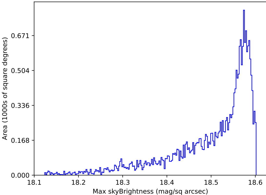
too_5_4v3.4_10yrs All sky y band: Max skyBrightness
